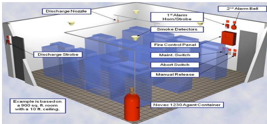
DSS-P FIRE SUPPRESSION SYSTEM NOVEC 123
